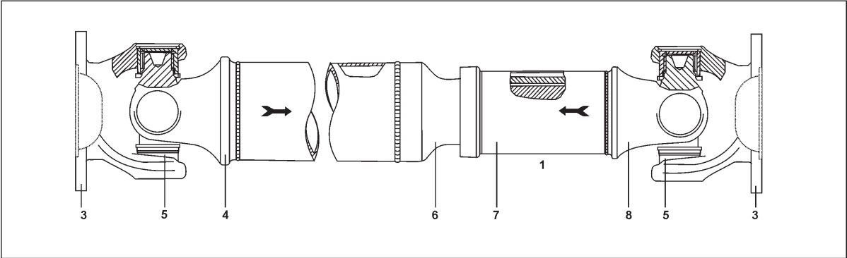
PROPELLER SHAFT FRONT (SPICER)
