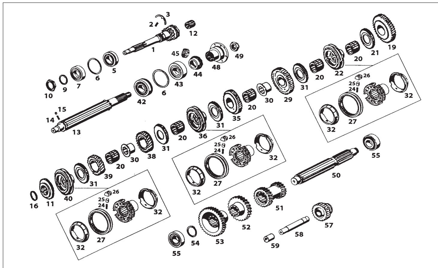
GEAR SHAFT AND GEAR (GBS 50)
