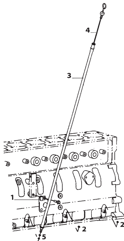
DIPSTICK
