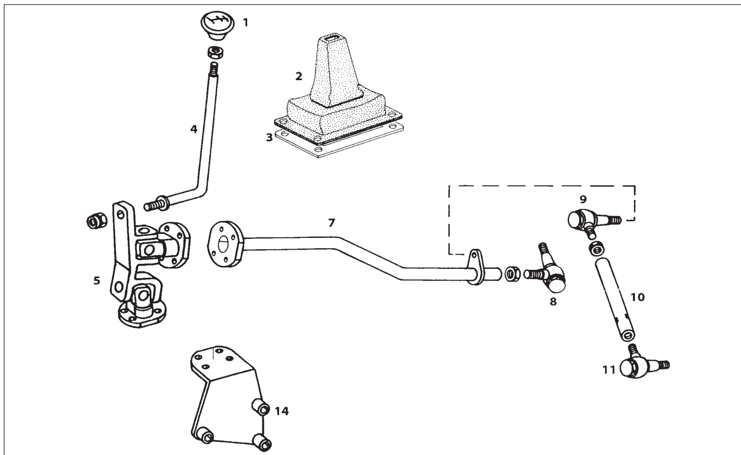
GEAR SHIFTING ARRANGEMENT (GBS 50)
